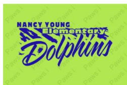
Script
